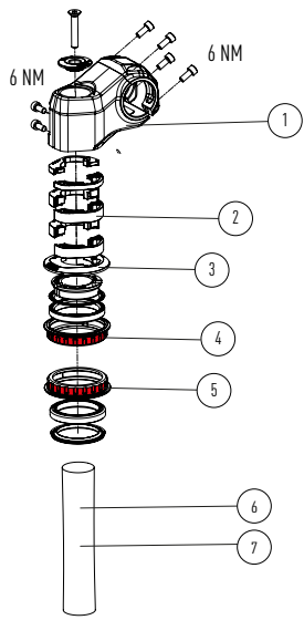
COCKPIT 30° WITHOUT BLOCK LOCK
